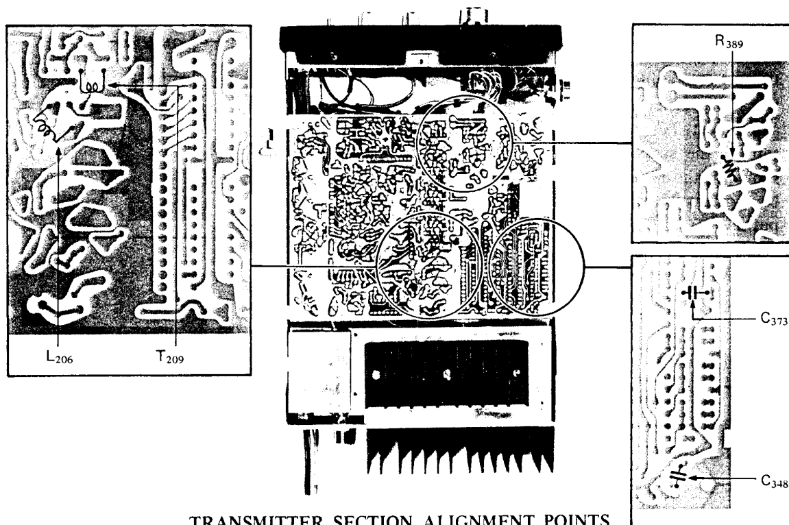
TRANSMITTER SECTION ALIGNMENT POINTS
