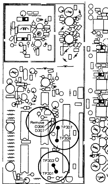
BAND E, E(12.5 kHz)
