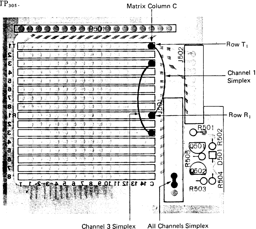
Figure 2-1 Viewed from solder side
