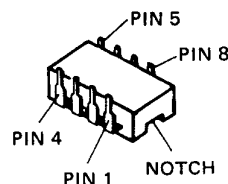
μPB551C
