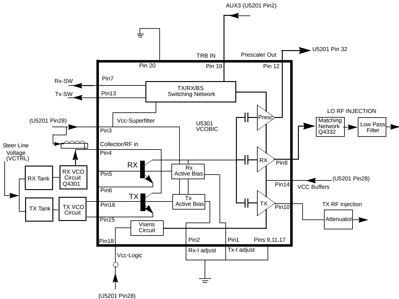
Figure 2-4 UHF VCO Block Diagram
